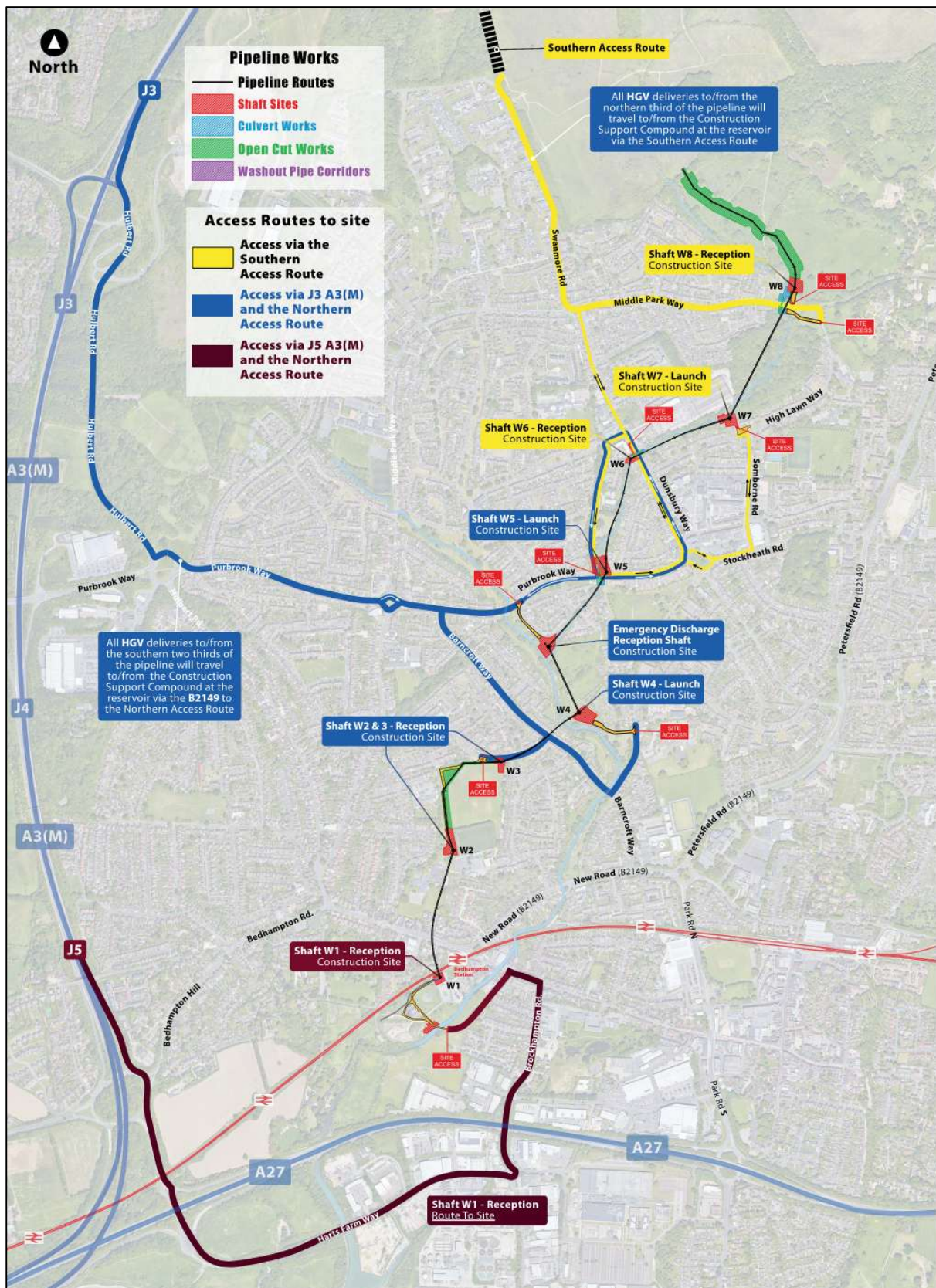
Map of overall construction traffic routes
