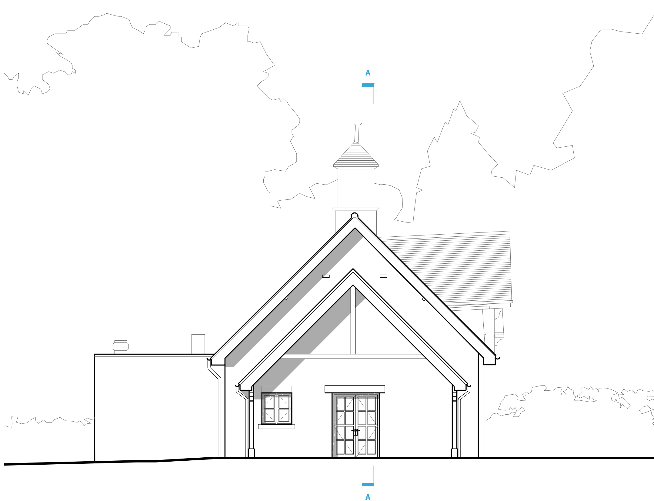
WEST ELEVATION
